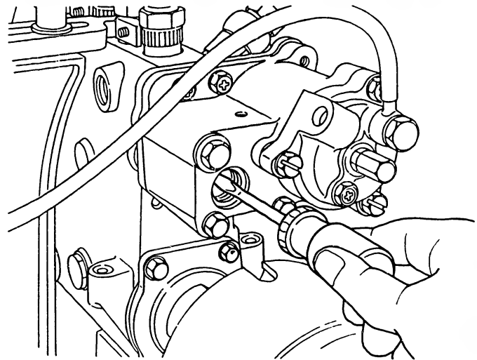
Fig. 107 Adjusting the boost compensator stroke
